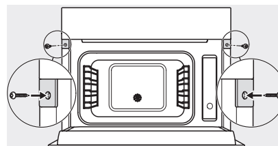
Installation DG, DGM, DGC XL, ESW7x10, EVS7010, installation drawings
