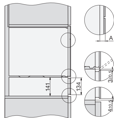
Side view DG, DGM, ESW7x10, EVS7010 installation drawings
